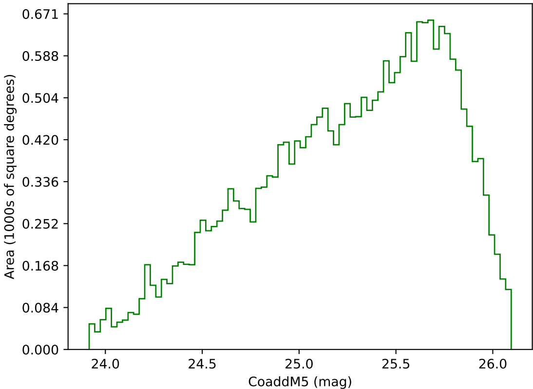
ddf_acor_sf30_lsf40_lsr20_v3.4_10yrs Yr 3-4 g band: CoaddM5
