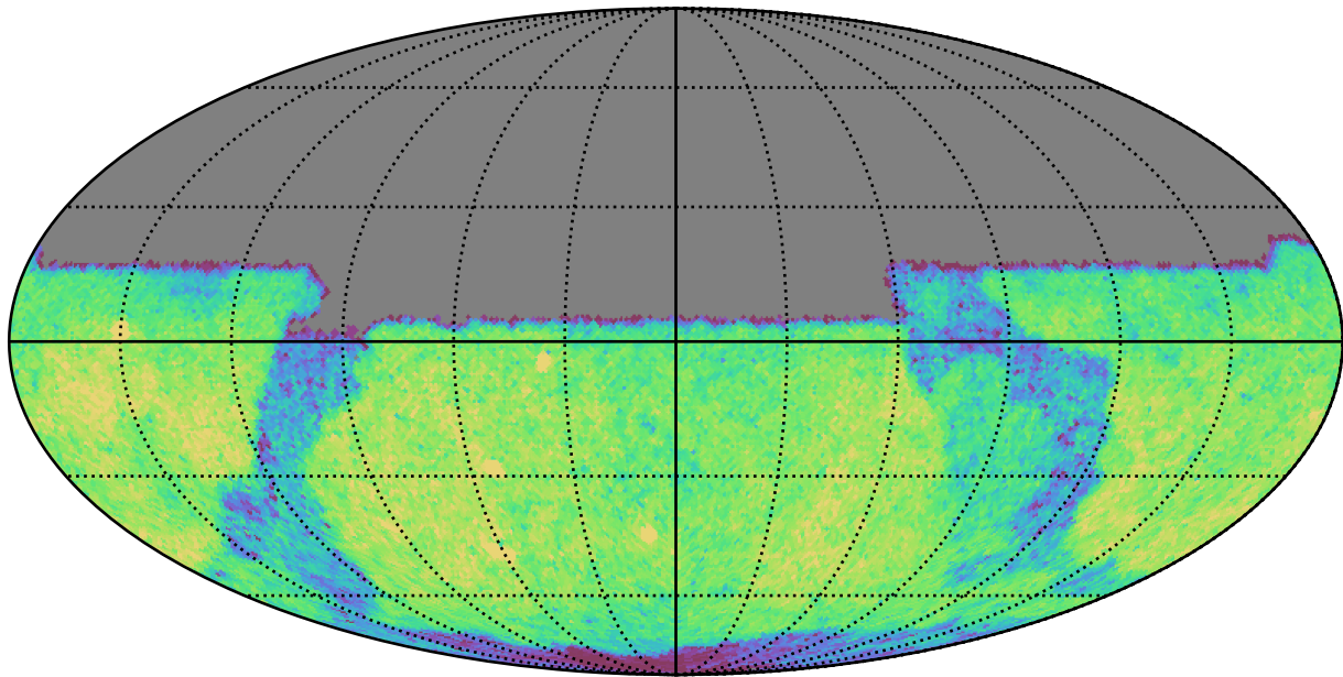
ddf_acor_sf30_lsf40_lsr20_v3.4_10yrs Yr 1 y band: CoaddM5
