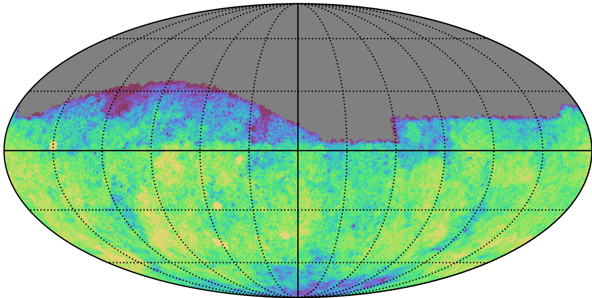
ddf_acor_sf30_lsf40_lsr20_v3.4_10yrs Yr 1 g band: CoaddM5
