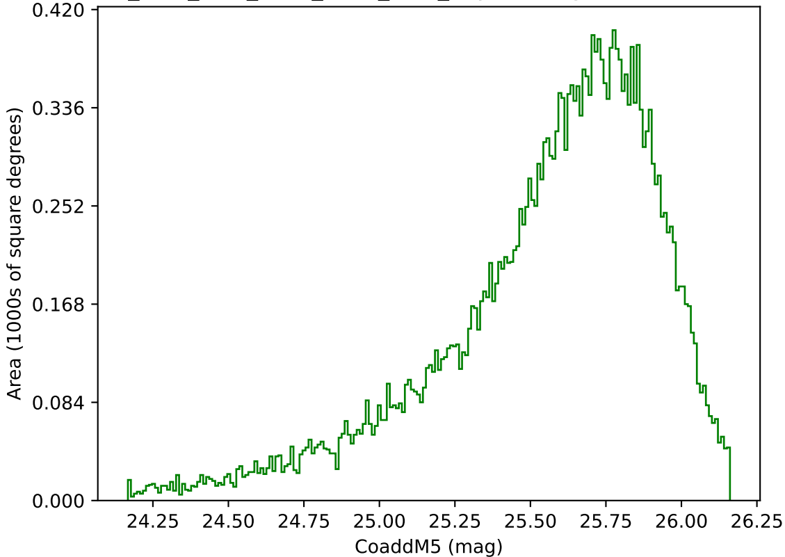
ddf_acor_sf30_lsf40_lsr20_v3.4_10yrs Yr 1 g band: CoaddM5
