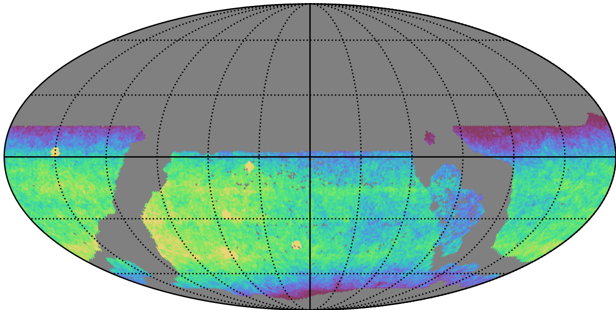
ddf_acor_sf30_lsf40_lsr20_v3.4_10yrs WFD z band: CoaddM5
