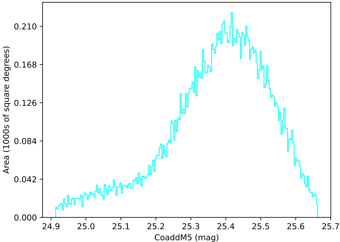
ddf_acor_sf30_lsf40_lsr20_v3.4_10yrs WFD u band: CoaddM5
