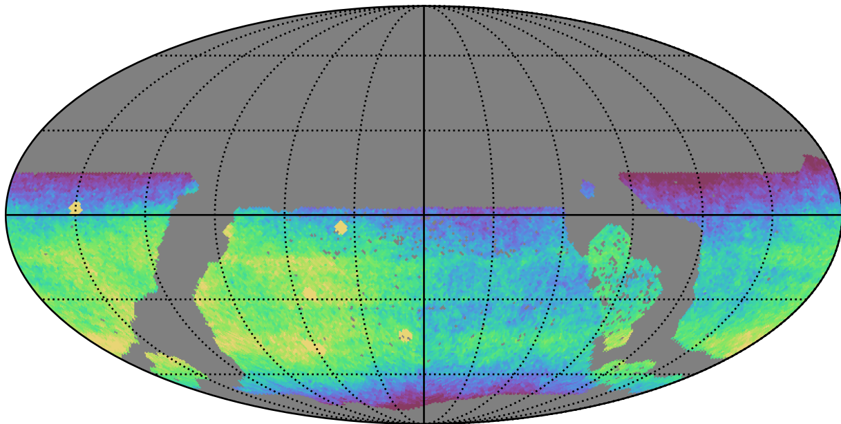
ddf_acor_sf30_lsf40_lsr20_v3.4_10yrs WFD r band: CoaddM5
