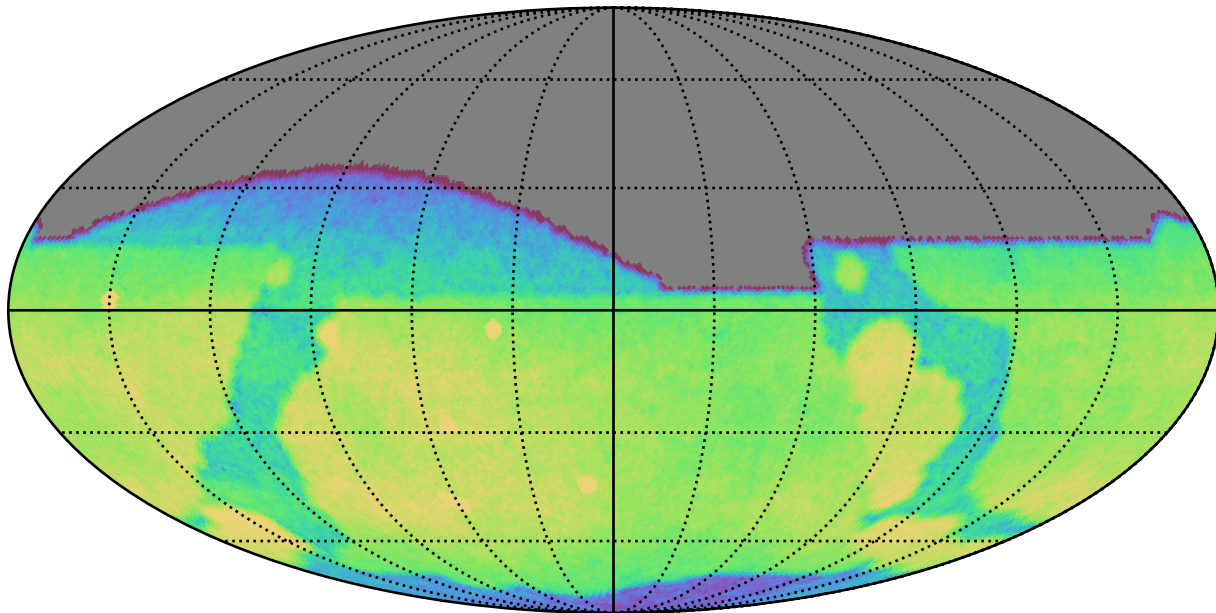
ddf_acor_sf30_lsf40_lsr20_v3.4_10yrs All sky g band: CoaddM5
