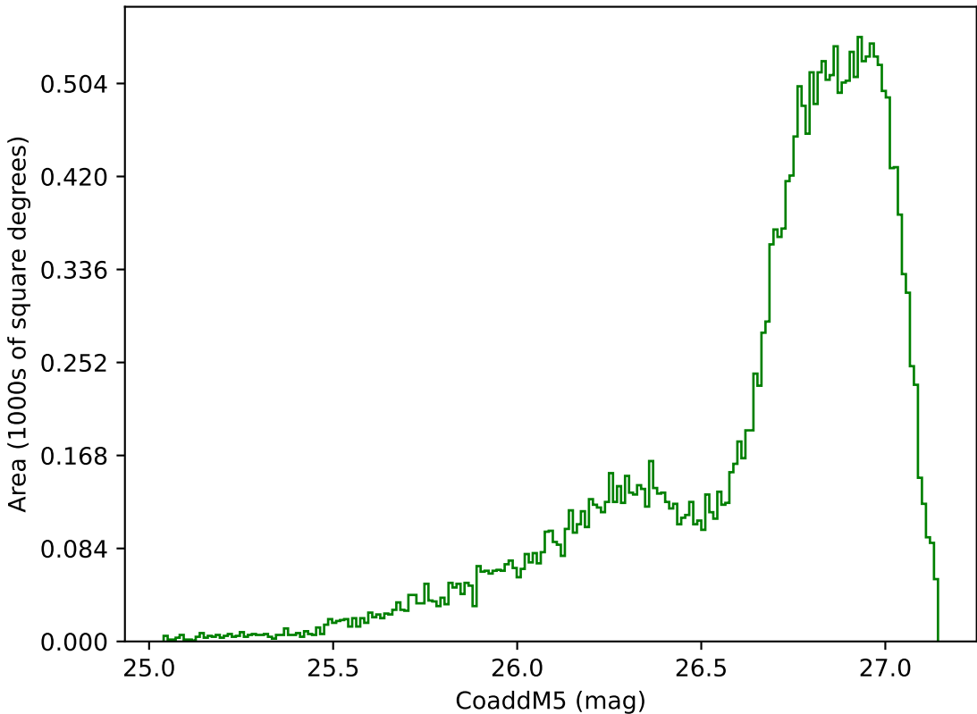
ddf_acor_sf30_lsf40_lsr20_v3.4_10yrs All sky g band: CoaddM5
