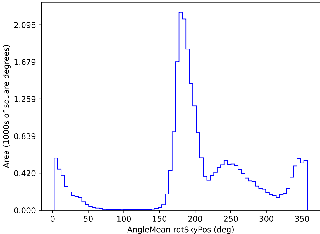
ddf_acor_sf30_lsf40_lsr20_v3.4_10yrs All sky i band: AngleMean rotSkyPos
