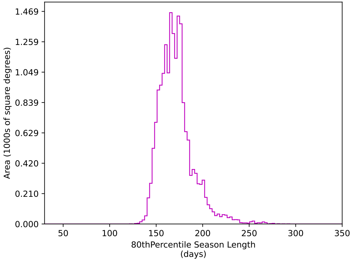
ddf_acor_sf30_lsf40_lsr20_v3.4_10yrs WFD z band: 80thPercentile Season Length
