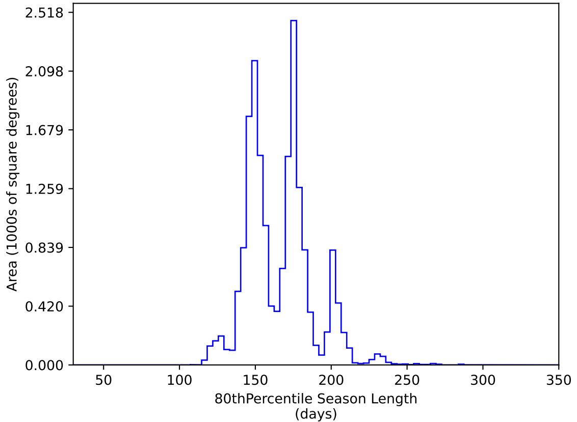
ddf_acor_sf30_lsf40_lsr20_v3.4_10yrs WFD y band: 80thPercentile Season Length
