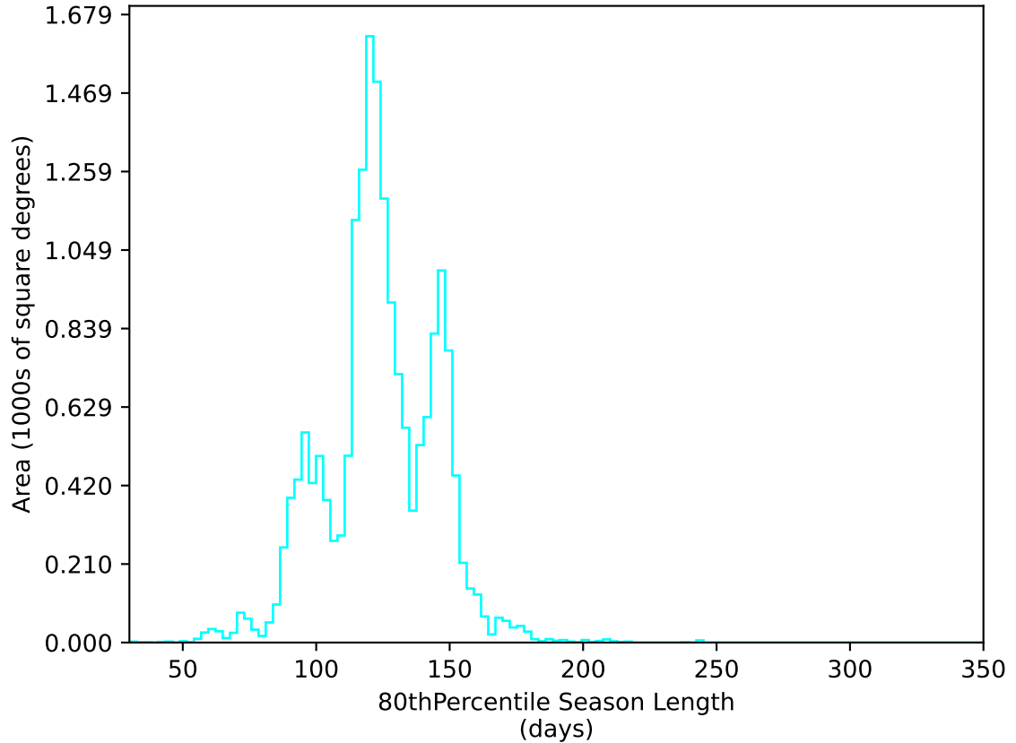
ddf_acor_sf30_lsf40_lsr20_v3.4_10yrs WFD u band: 80thPercentile Season Length
