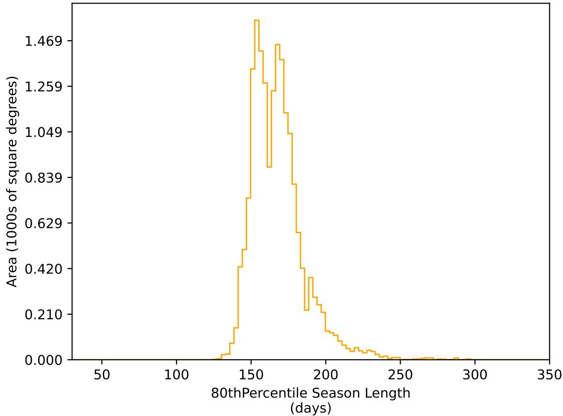
ddf_acor_sf30_lsf40_lsr20_v3.4_10yrs WFD r band: 80thPercentile Season Length
