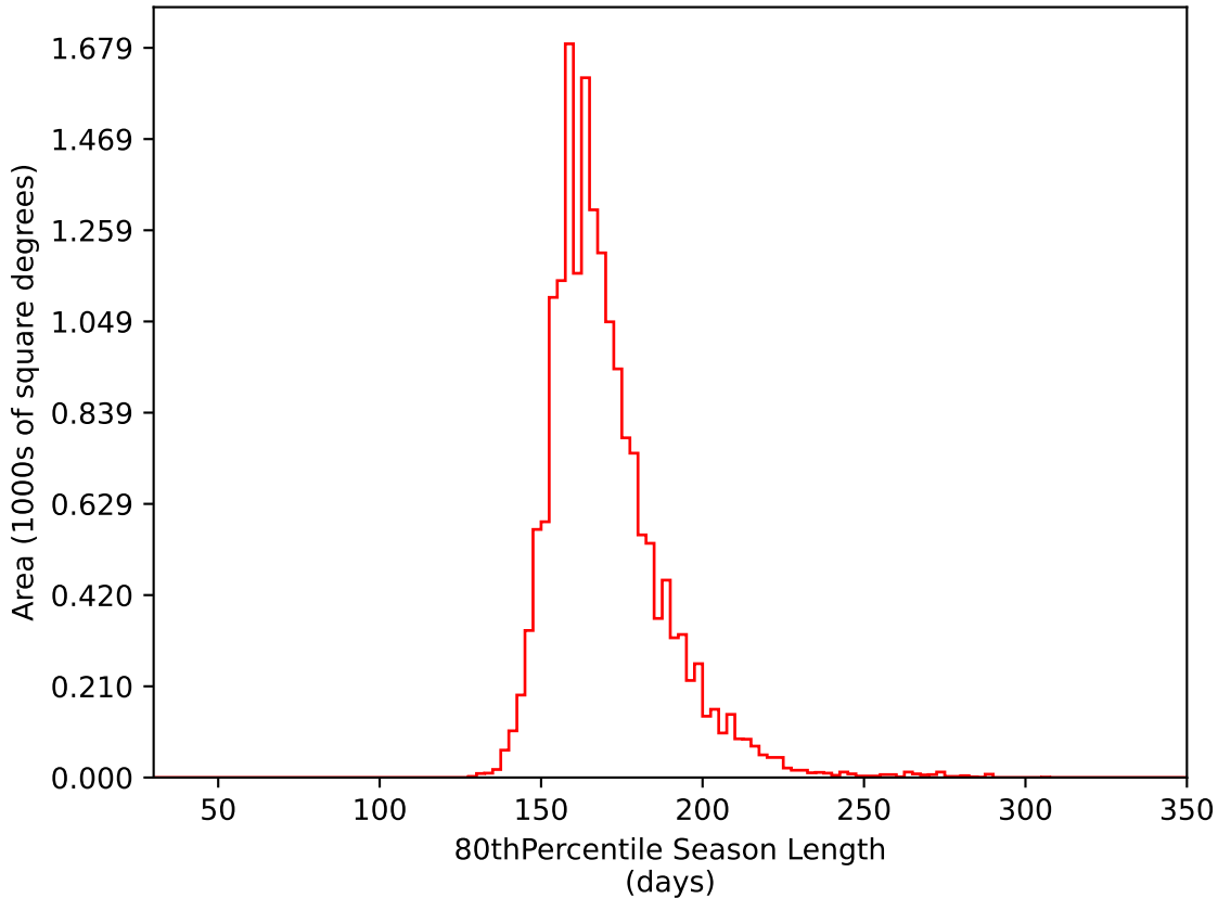
ddf_acor_sf30_lsf40_lsr20_v3.4_10yrs WFD i band: 80thPercentile Season Length
