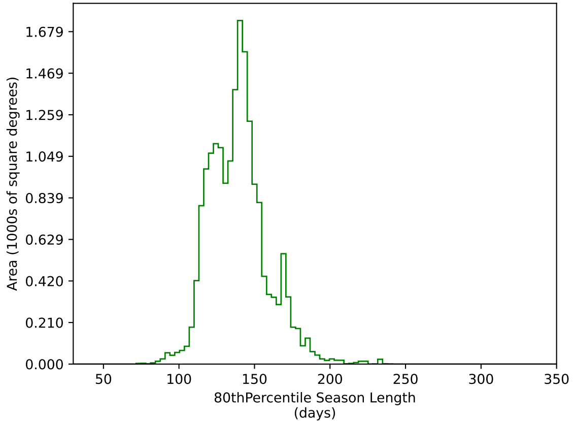
ddf_acor_sf30_lsf40_lsr20_v3.4_10yrs WFD g band: 80thPercentile Season Length
