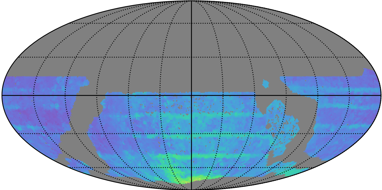
ddf_acor_sf30_lsf40_lsr20_v3.4_10yrs WFD all bands: 80thPercentile Season Length
