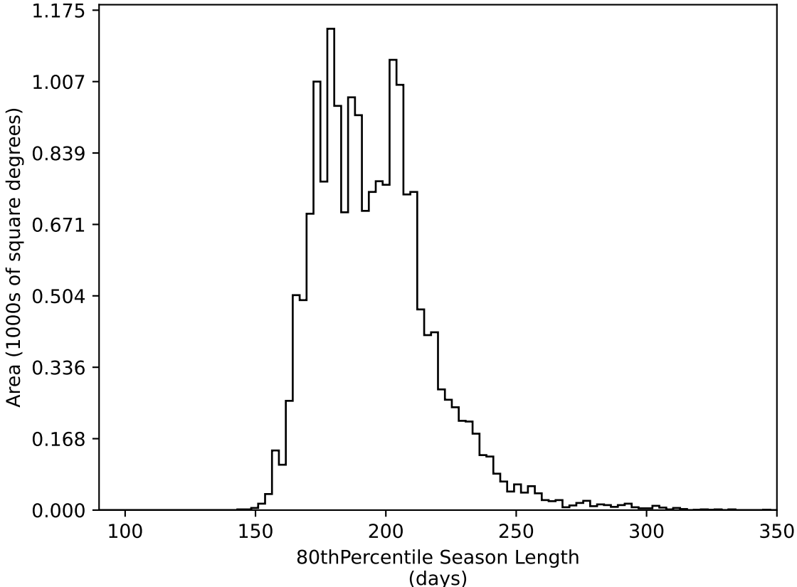
ddf_acor_sf30_lsf40_lsr20_v3.4_10yrs WFD all bands: 80thPercentile Season Length
