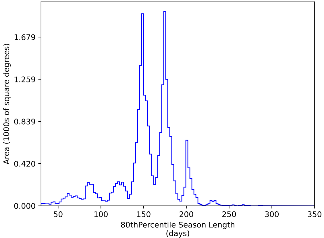
ddf_acor_sf30_lsf40_lsr20_v3.4_10yrs All sky y band: 80thPercentile Season Length
