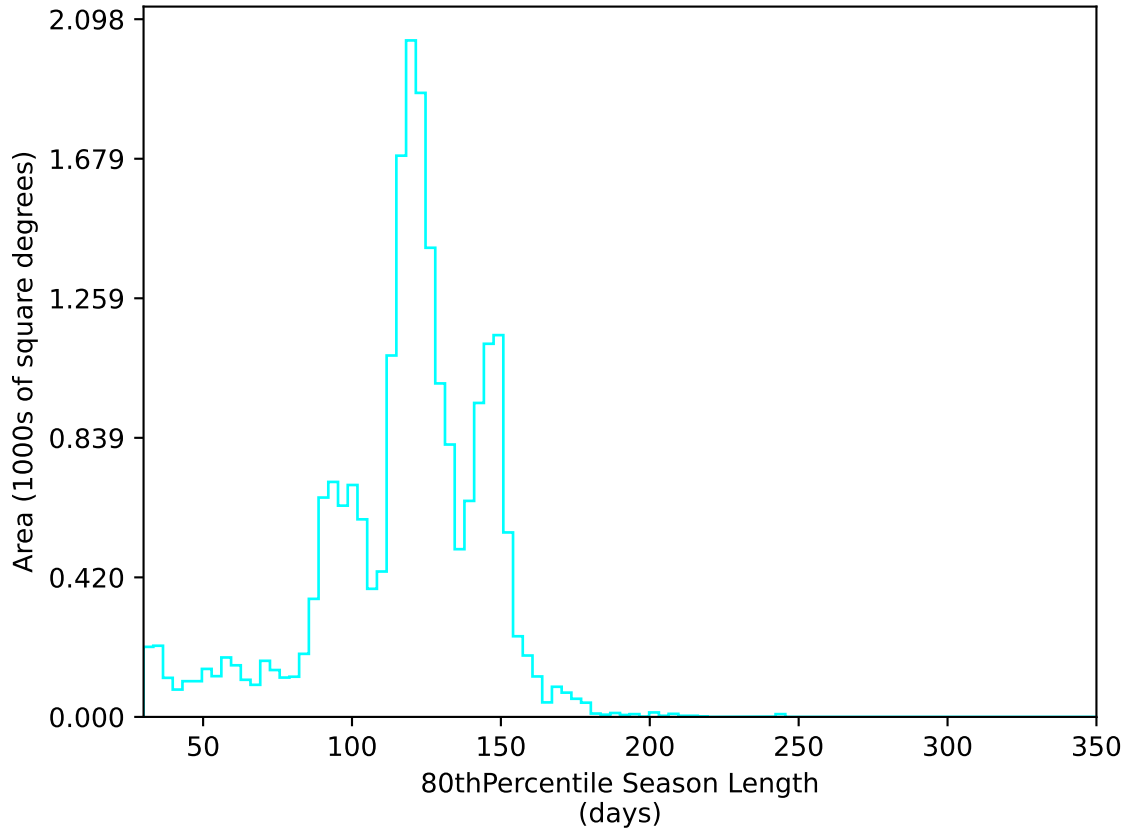
ddf_acor_sf30_lsf40_lsr20_v3.4_10yrs All sky u band: 80thPercentile Season Length
