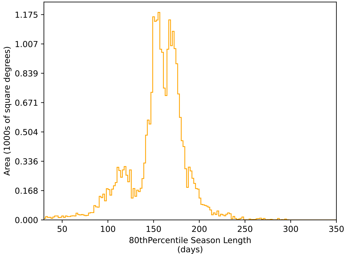
ddf_acor_sf30_lsf40_lsr20_v3.4_10yrs All sky r band: 80thPercentile Season Length
