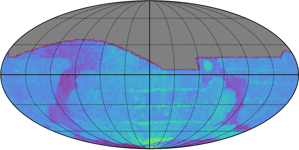
ddf_acor_sf30_lsf40_lsr20_v3.4_10yrs All sky i band: 80thPercentile Season Length
