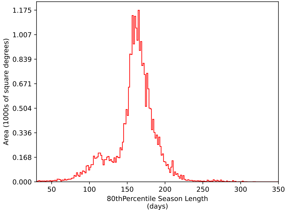
ddf_acor_sf30_lsf40_lsr20_v3.4_10yrs All sky i band: 80thPercentile Season Length
