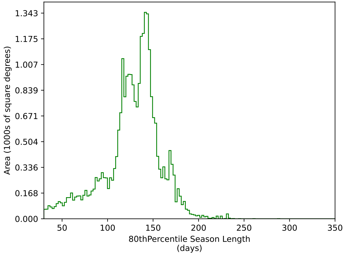
ddf_acor_sf30_lsf40_lsr20_v3.4_10yrs All sky g band: 80thPercentile Season Length
