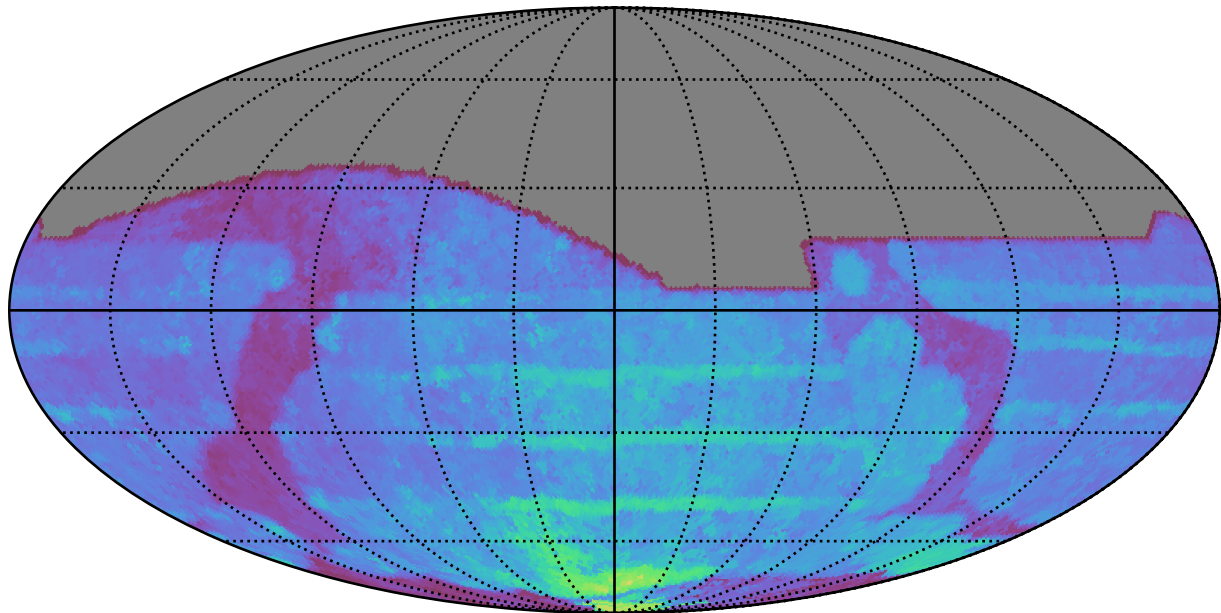
ddf_acor_sf30_lsf40_lsr20_v3.4_10yrs All sky all bands: 80thPercentile Season Length
