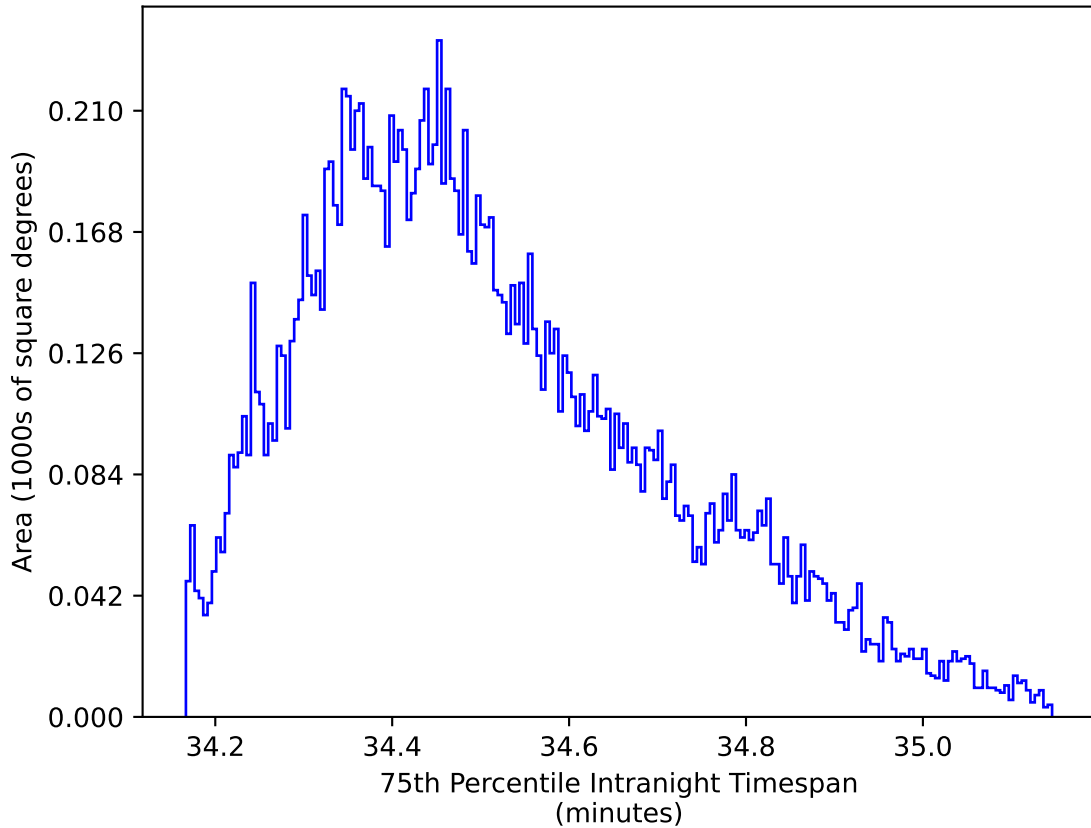
ddf_acor_sf30_lsf40_lsr20_v3.4_10yrs WFD zy bands: 75th Percentile Intranight Timespan
