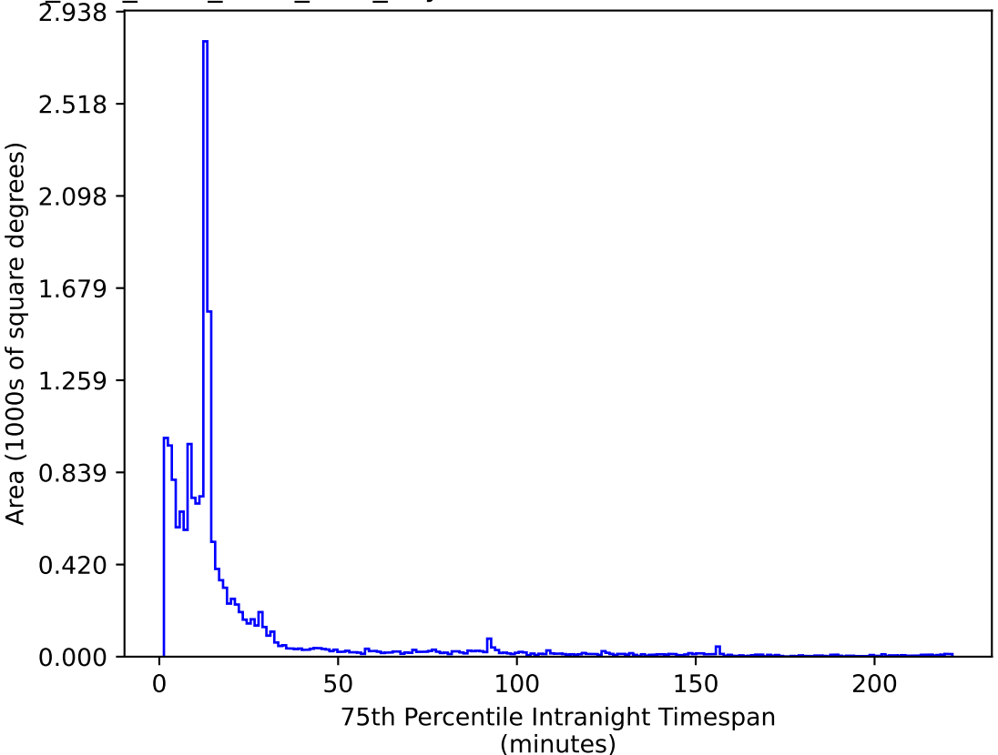
ddf_acor_sf30_lsf40_lsr20_v3.4_10yrs WFD z band: 75th Percentile Intranight Timespan
