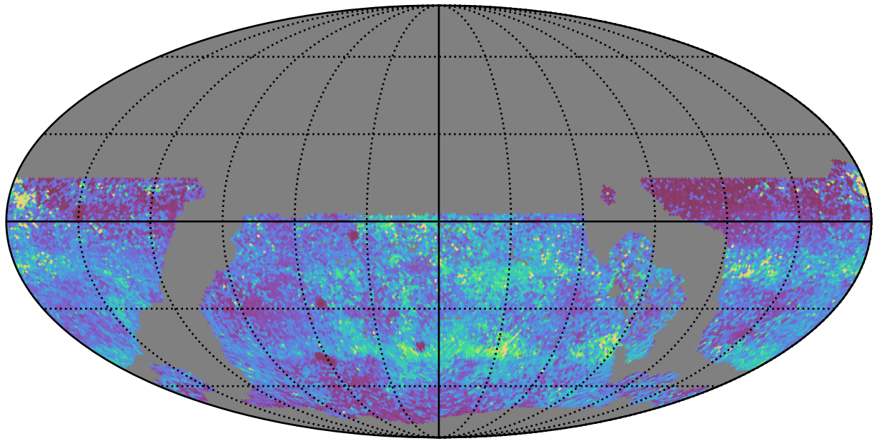
ddf_acor_sf30_lsf40_lsr20_v3.4_10yrs WFD y band: 75th Percentile Intranight Timespan
