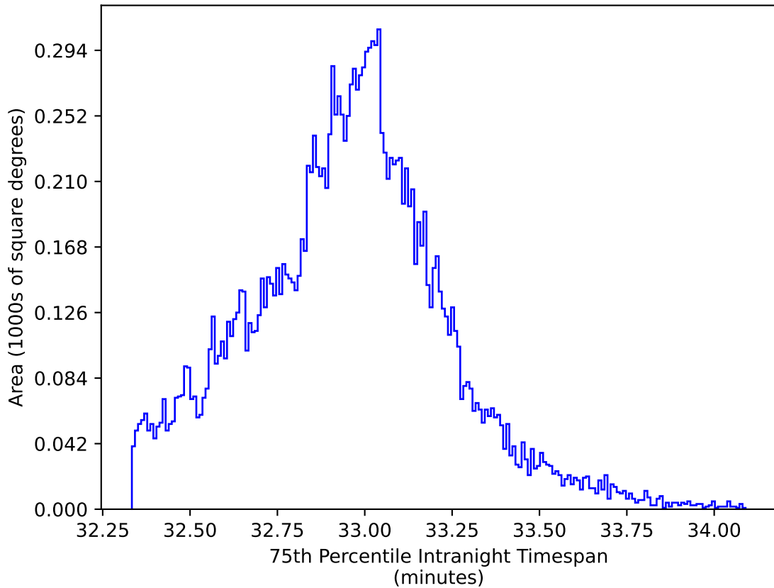
ddf_acor_sf30_lsf40_lsr20_v3.4_10yrs WFD y band: 75th Percentile Intranight Timespan
