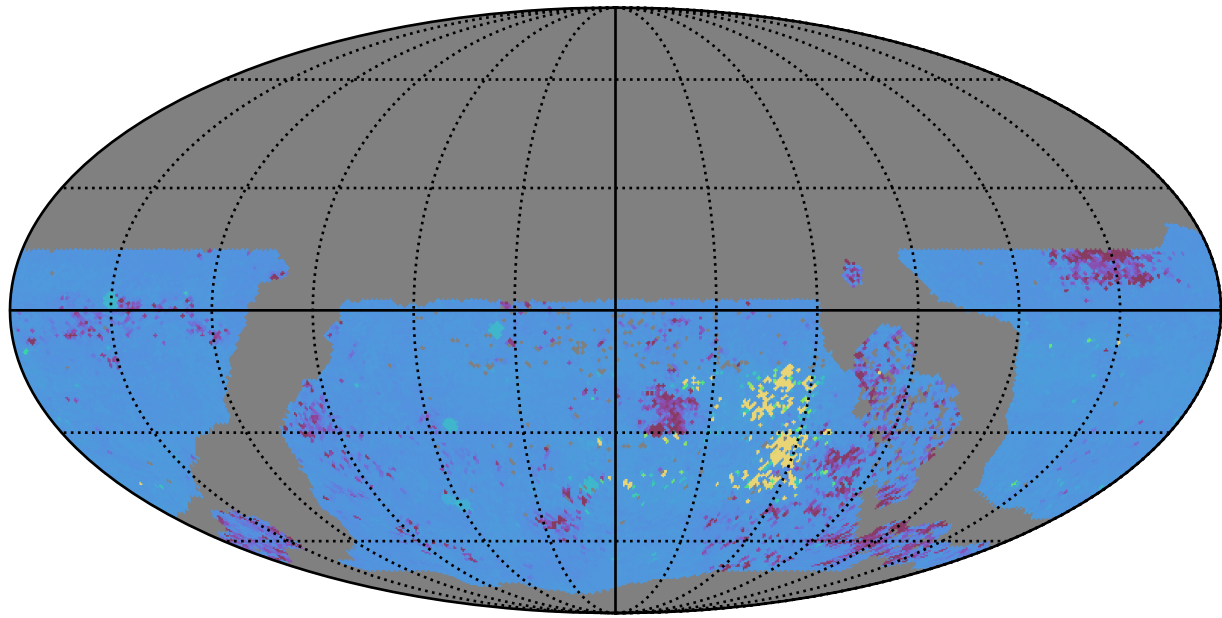
ddf_acor_sf30_lsf40_lsr20_v3.4_10yrs WFD ug bands: 75th Percentile Intranight Timespan
