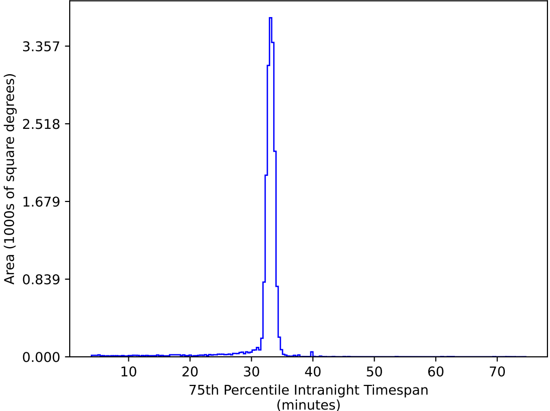
ddf_acor_sf30_Isf40_Isr20_v3.4_10yrs WFD ug bands: 75th Percentile Intranight Timespan
