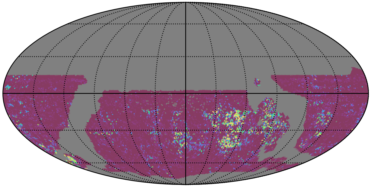
ddf_acor_sf30_lsf40_lsr20_v3.4_10yrs WFD u band: 75th Percentile Intranight Timespan
