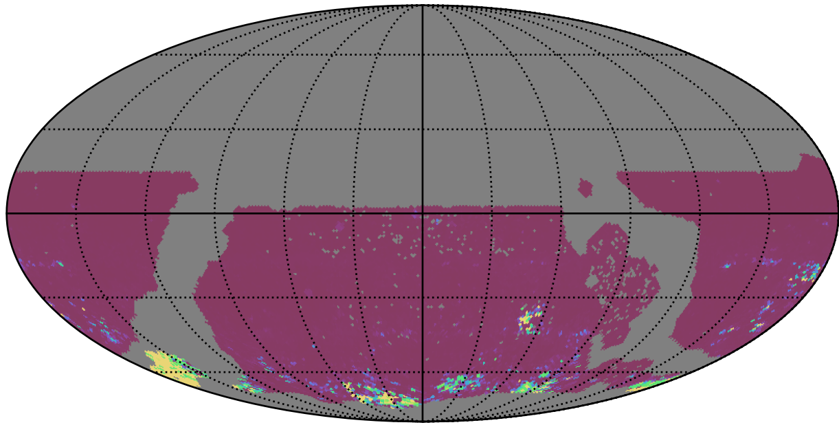
ddf_acor_sf30_lsf40_lsr20_v3.4_10yrs WFD ri bands: 75th Percentile Intranight Timespan
