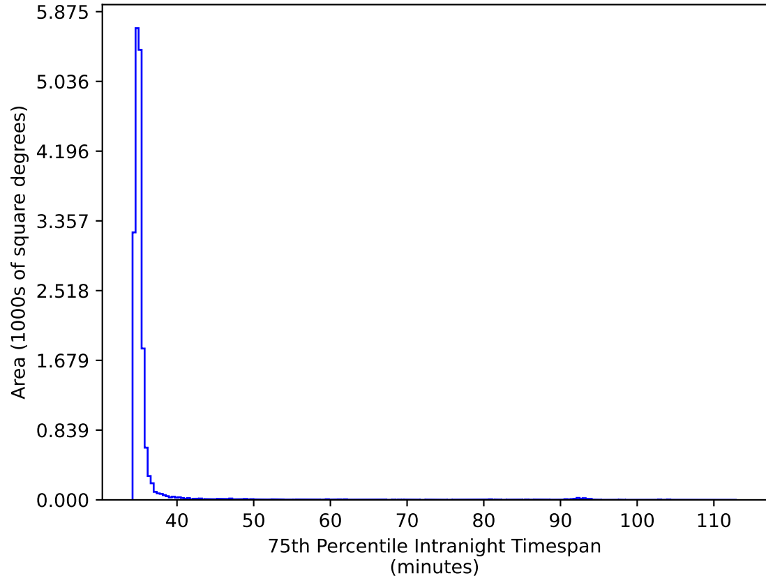
ddf_acor_sf30_lsf40_lsr20_v3.4_10yrs WFD ri bands: 75th Percentile Intranight Timespan
