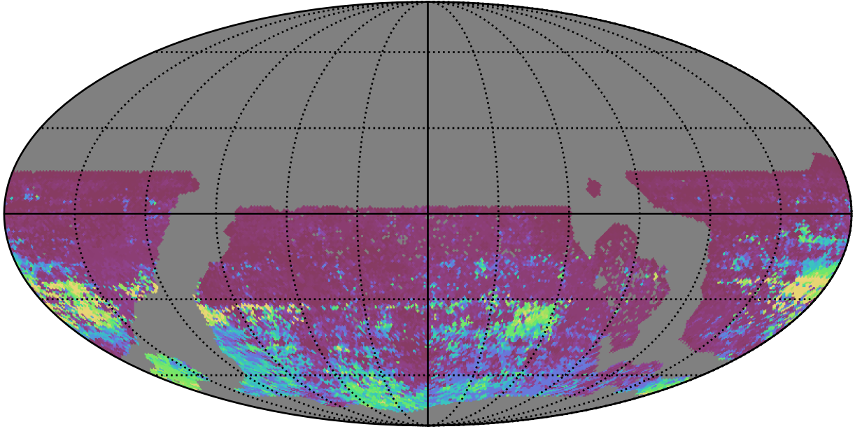
ddf_acor_sf30_lsf40_lsr20_v3.4_10yrs WFD r band: 75th Percentile Intranight Timespan
