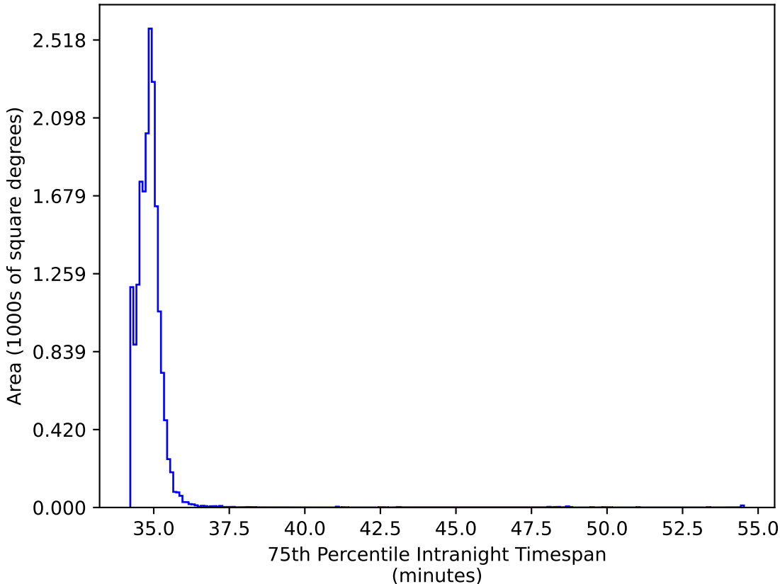
ddf_acor_sf30_lsf40_lsr20_v3.4_10yrs WFD iz bands: 75th Percentile Intranight Timespan
