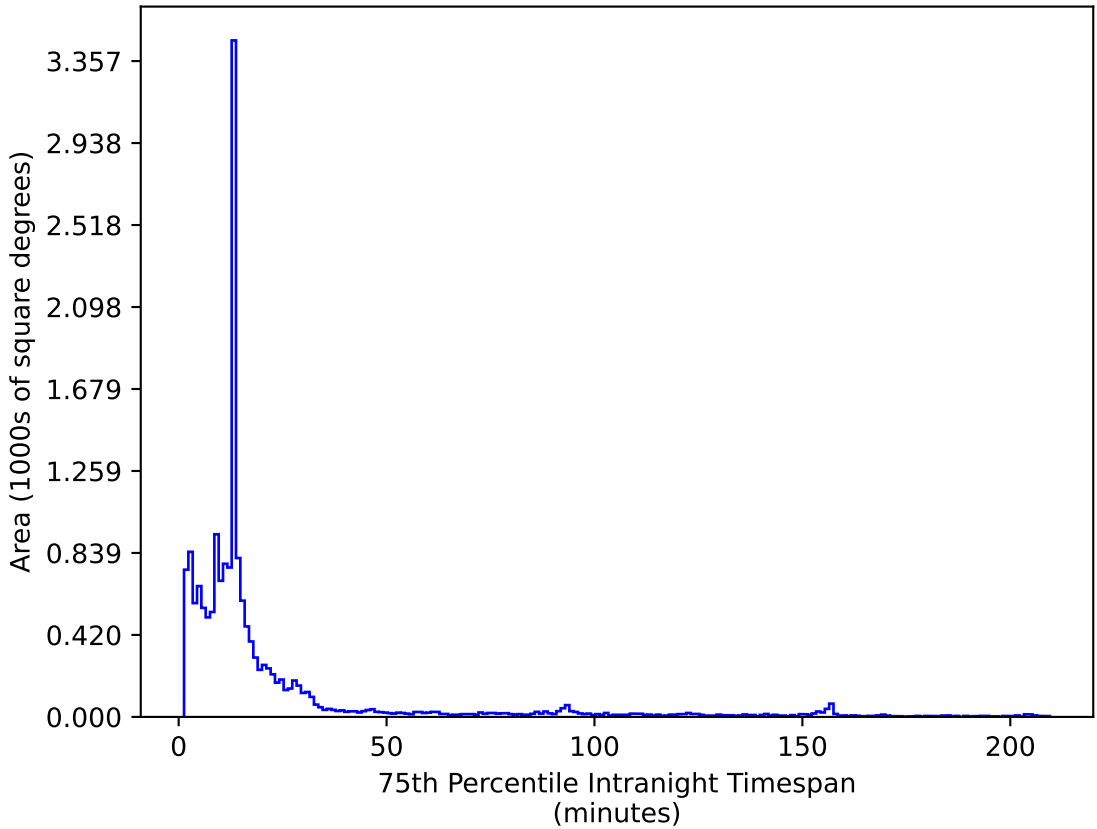
ddf_acor_sf30_lsf40_lsr20_v3.4_10yrs WFD i band: 75th Percentile Intranight Timespan
