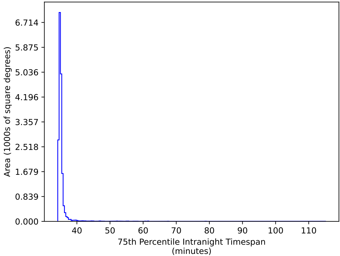
ddf_acor_sf30_lsf40_lsr20_v3.4_10yrs WFD gr bands: 75th Percentile Intranight Timespan
