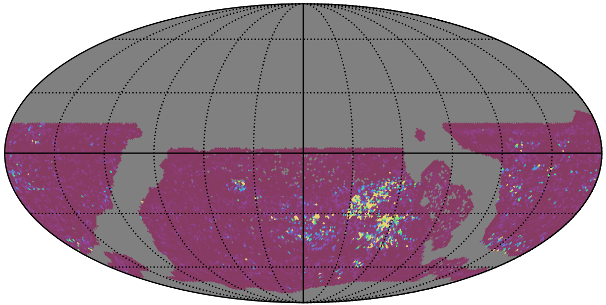
ddf_acor_sf30_lsf40_lsr20_v3.4_10yrs WFD g band: 75th Percentile Intranight Timespan
