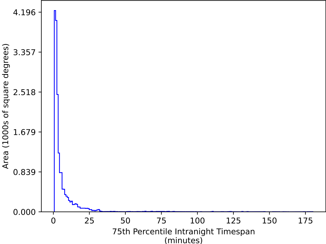
ddf_acor_sf30_lsf40_lsr20_v3.4_10yrs WFD g band: 75th Percentile Intranight Timespan
