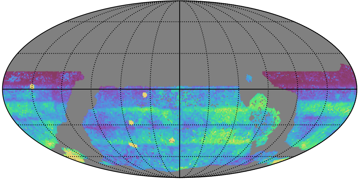
ddf_acor_sf30_lsf40_lsr20_v3.4_10yrs WFD all bands: 75th Percentile Intranight Timespan
