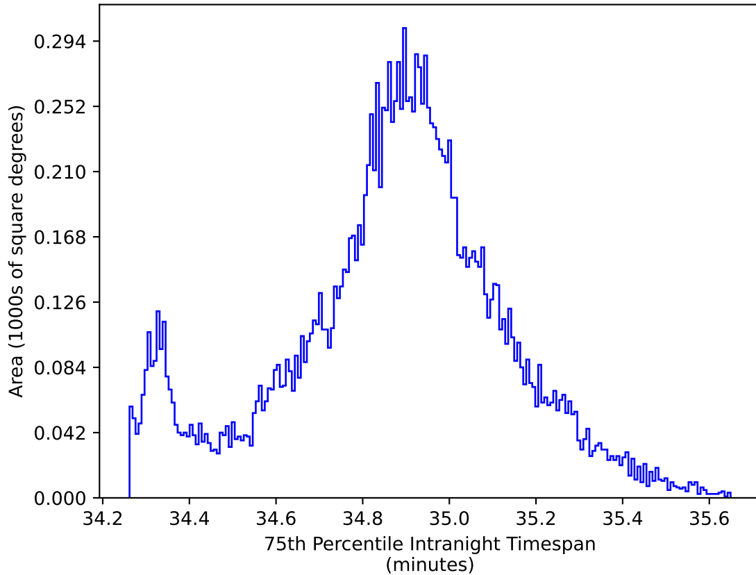
ddf_acor_sf30_Isf40_Isr20_v3.4_10yrs WFD all bands: 75th Percentile Intranight Timespan
