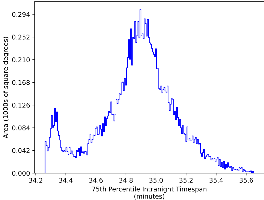
ddf_acor_sf30_ls40_lsr20_v3.4_10yrs WFD: 75th Percentile Intranight Timespan
