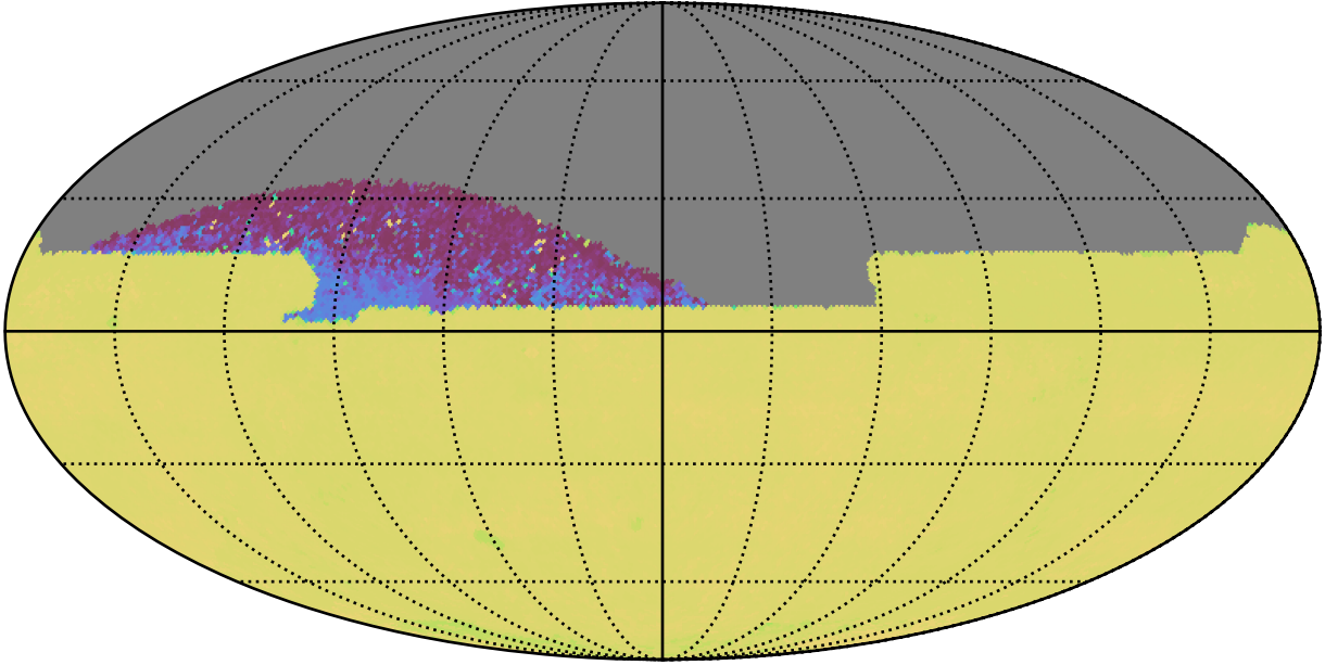
ddf_acor_sf30_lsf40_lsr20_v3.4_10yrs All sky zy bands: 75th Percentile Intranight Timespan
