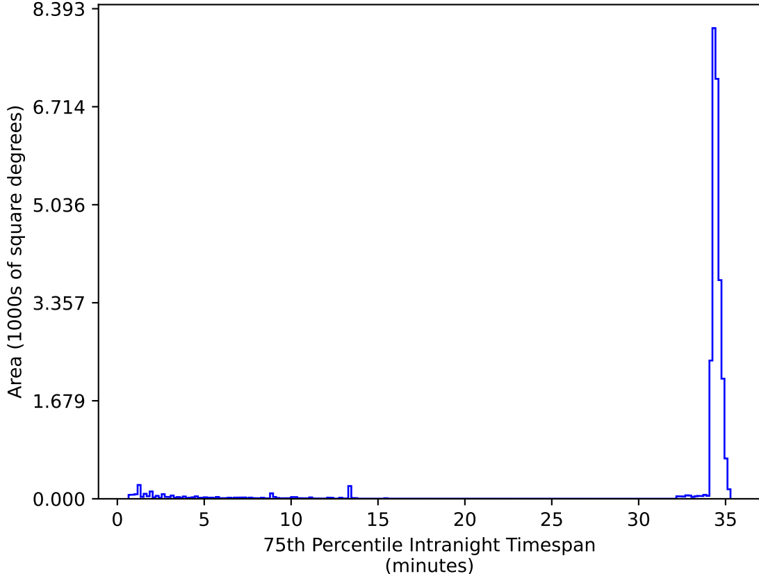
ddf_acor_sf30_lsf40_lsr20_v3.4_10yrs All sky zy bands: 75th Percentile Intranight Timespan
