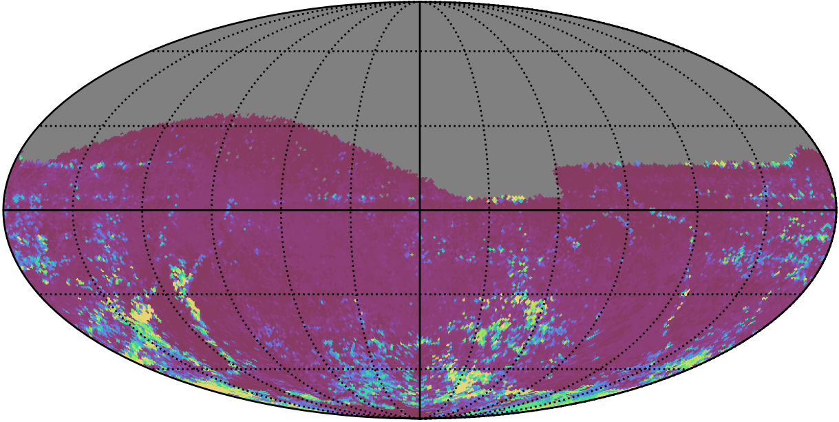
ddf_acor_sf30_lsf40_lsr20_v3.4_10yrs All sky z band: 75th Percentile Intranight Timespan
