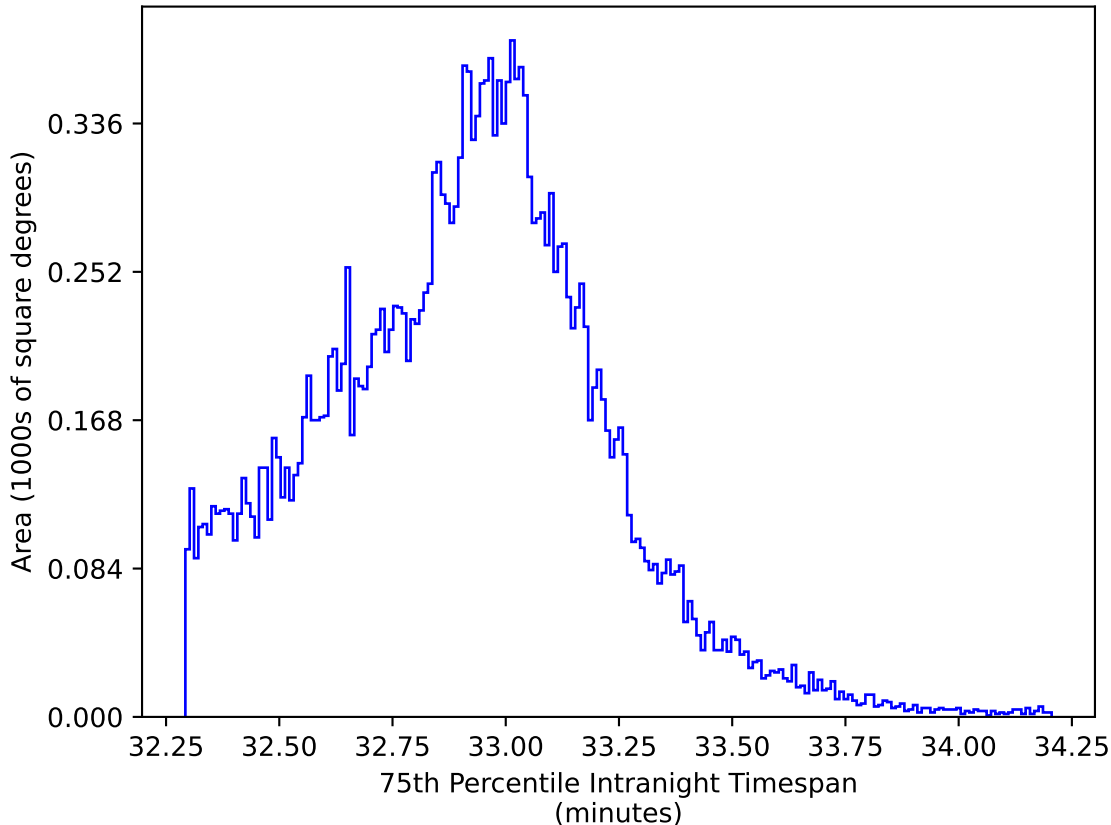
ddf_acor_sf30_lsf40_lsr20_v3.4_10yrs All sky y band: 75th Percentile Intranight Timespan
