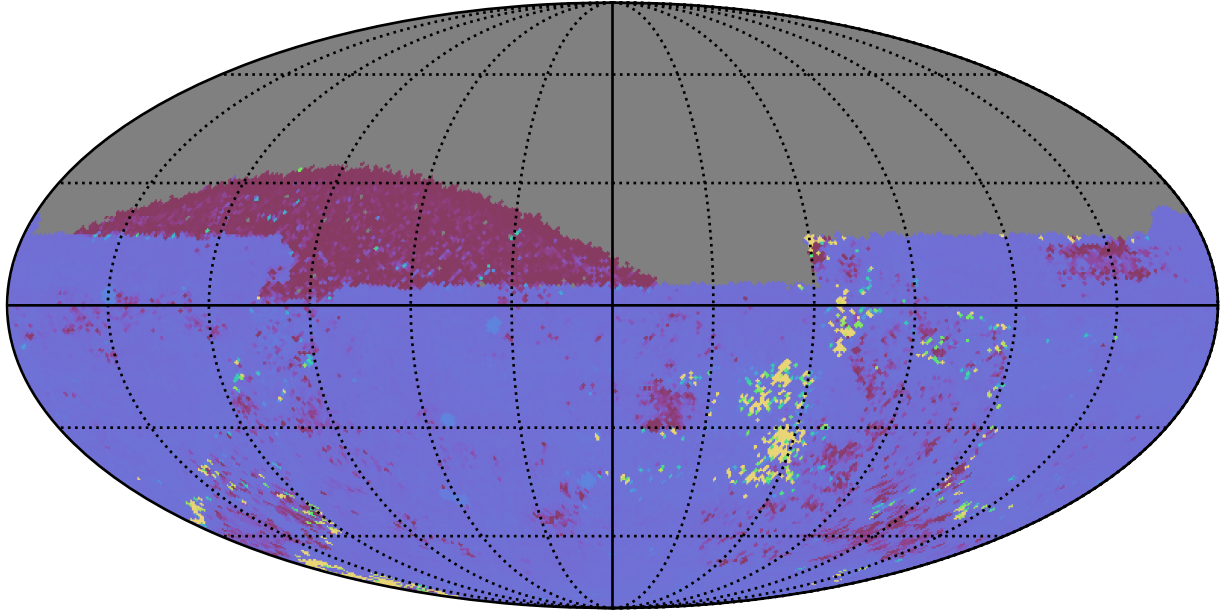
ddf_acor_sf30_lsf40_lsr20_v3.4_10yrs All sky ug bands: 75th Percentile Intranight Timespan
