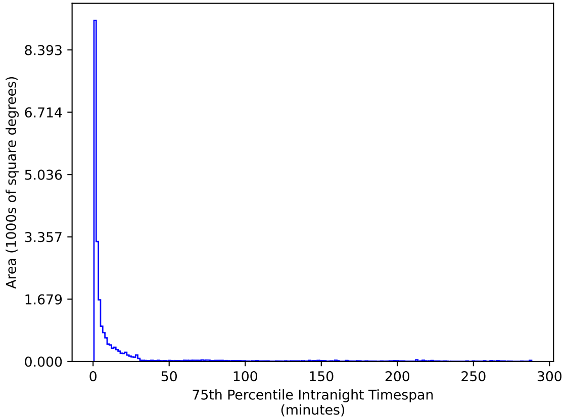
ddf_acor_sf30_lsf40_lsr20_v3.4_10yrs All sky u band: 75th Percentile Intranight Timespan
