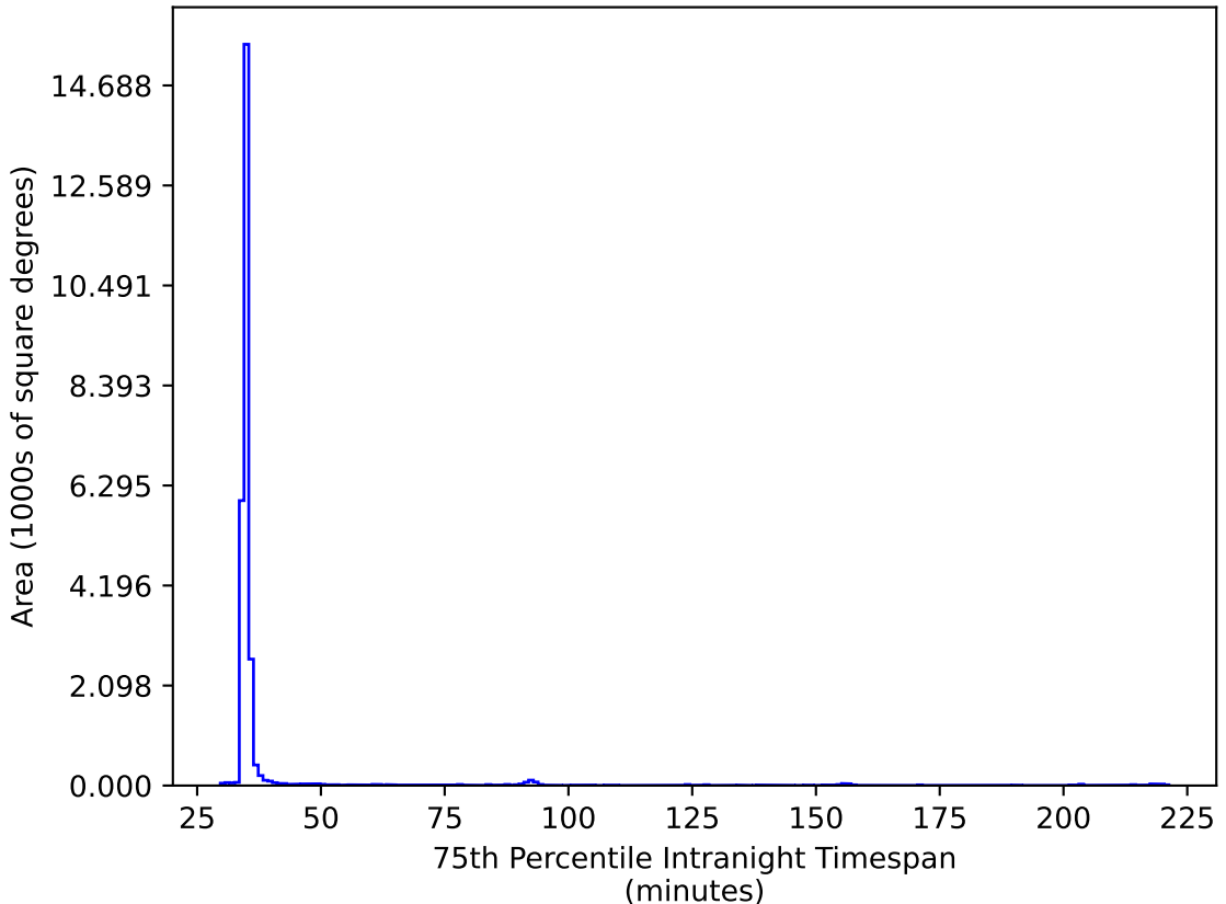
ddf_acor_sf30_lsf40_lsr20_v3.4_10yrs All sky ri bands: 75th Percentile Intranight Timespan
